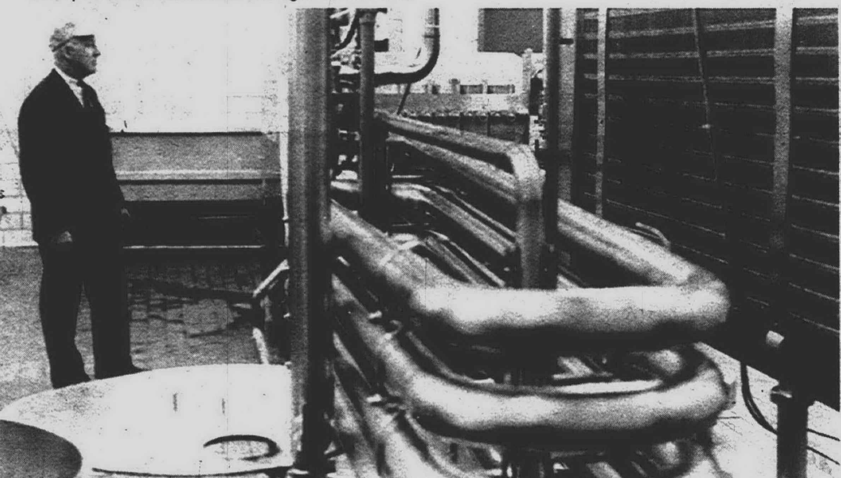
PASTEURIZING COILS — Kroger executive Bob Johnson stands beside the set of coils that holds all milk at 175 degrees Fahrenheit for 16 seconds.
