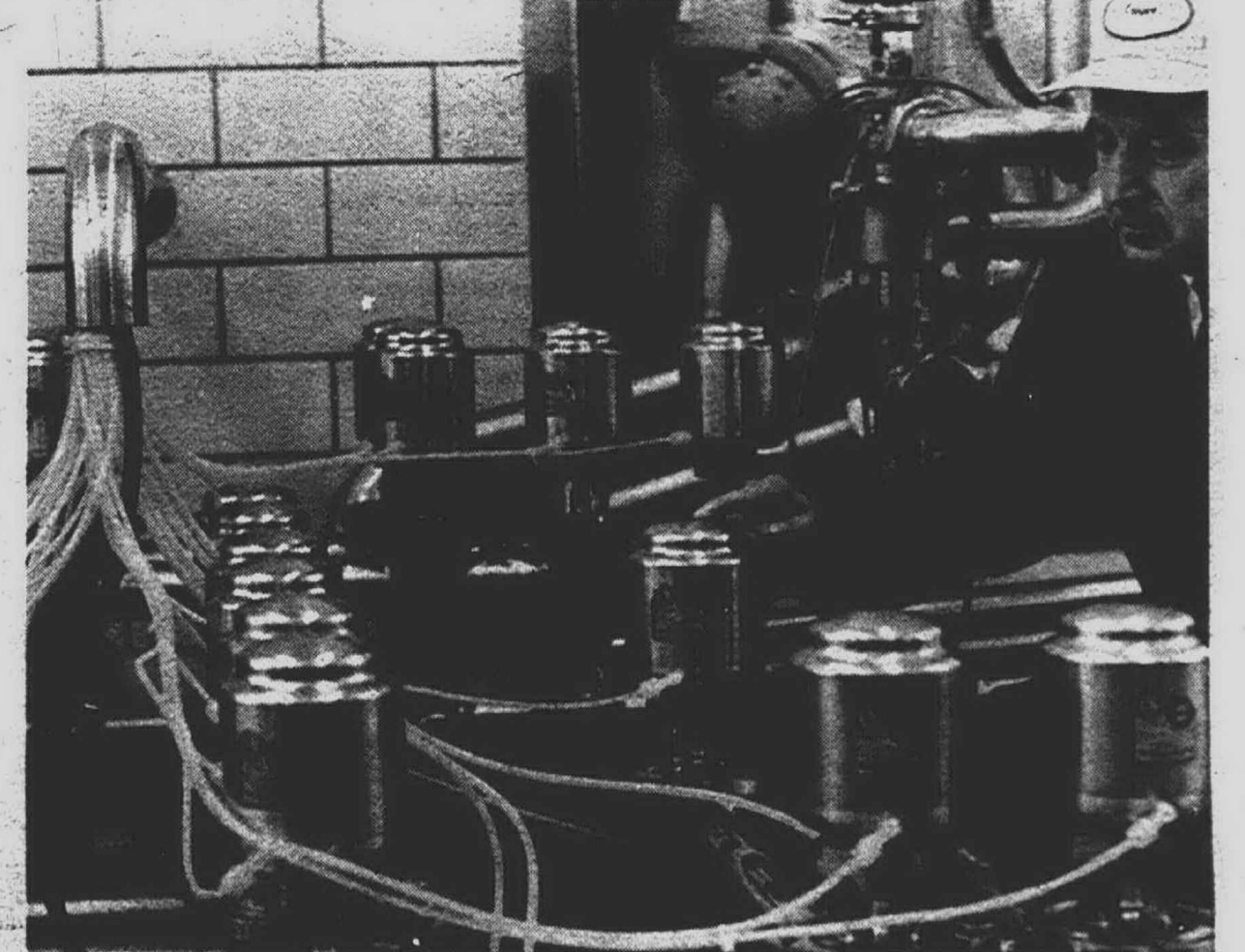
GRAND CENTRAL STATION — Each pipe in this complicated valve system Bob Johnson is checking leads some of the pasteurized milk through the process that makes it homogenized, buttermilk or chocolate.
